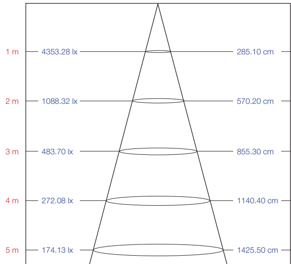
Height | Illuminance | Diameter Beam Angle: 109.90 Deg
