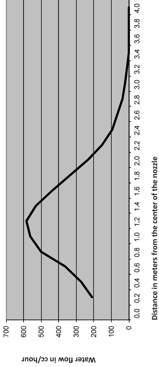
Spray pattern Pin nozzle Orange 4.35. ** 6
